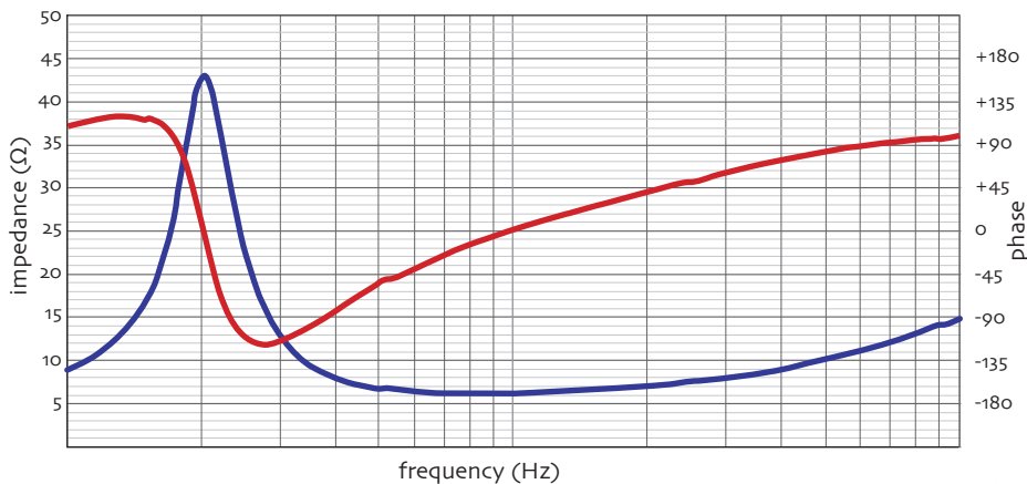
CSS SDX12 SubDuction Thiele/Small Parameters
